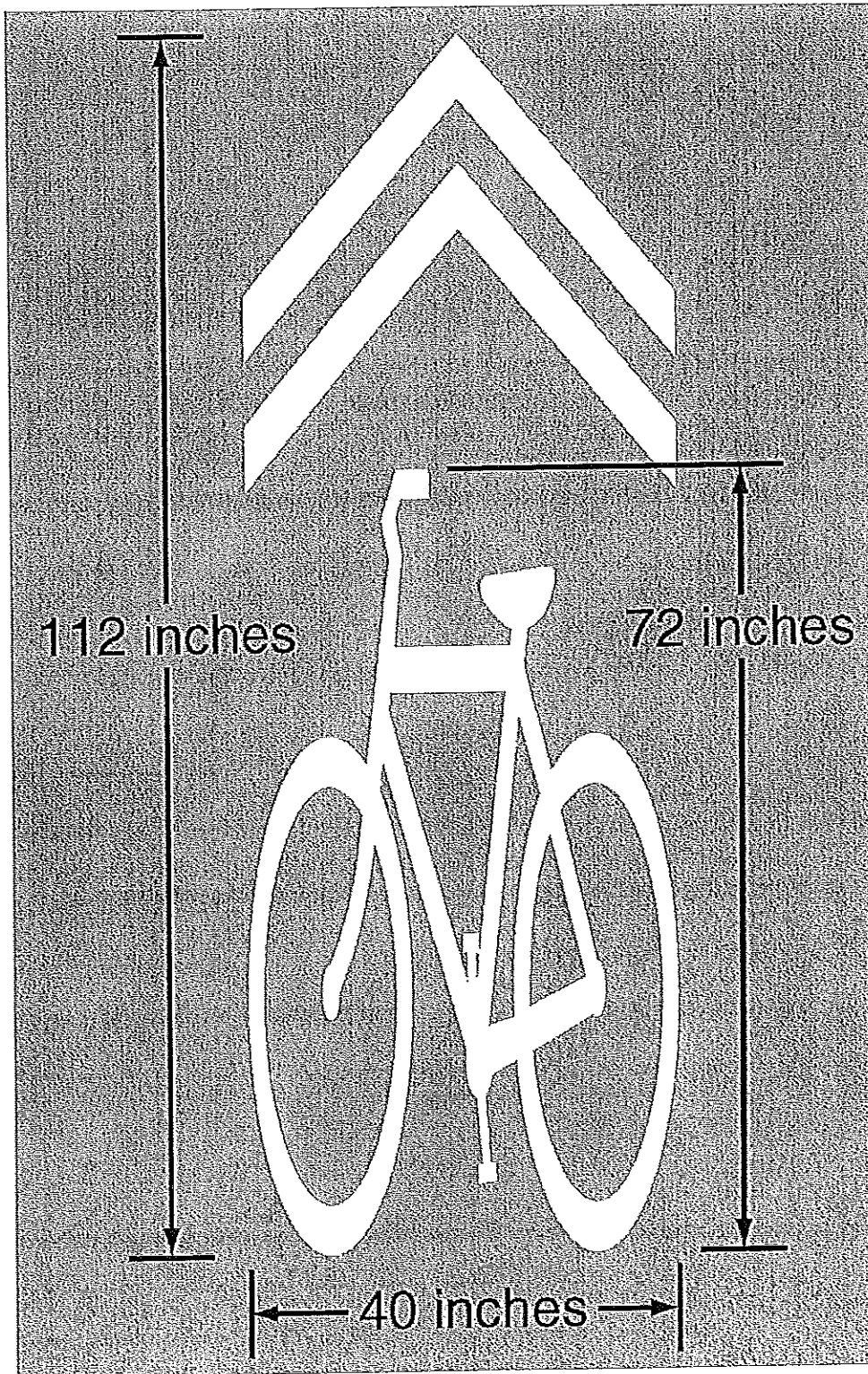
TRAFFIC MARKINGS, SHARED LANE SYMBOL, THERMOPLASTIC
